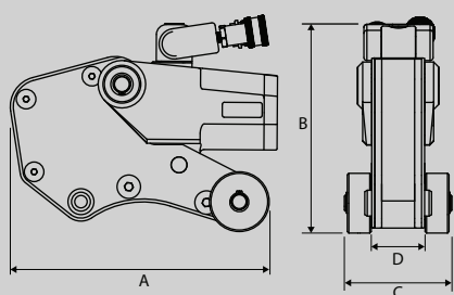
Tool Body
